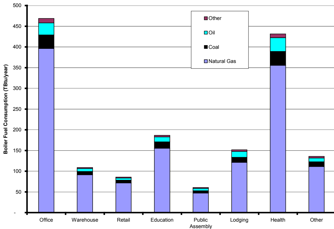
Figure 3-3 Energy Consumption in Commercial Boilers
